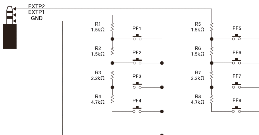
Fig. 78 KEYPAD Circuit Example
