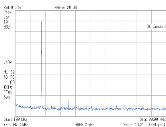
Fig. 22 DRV Output Characteristics 14.175 MHz 0 dBm Fig. 23 DRV Output Characteristics 14.175 MHz -10 dBm
