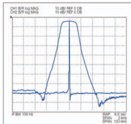
Fig. 6 Frequency response of the 270 Hz Bandwidth (Option)
