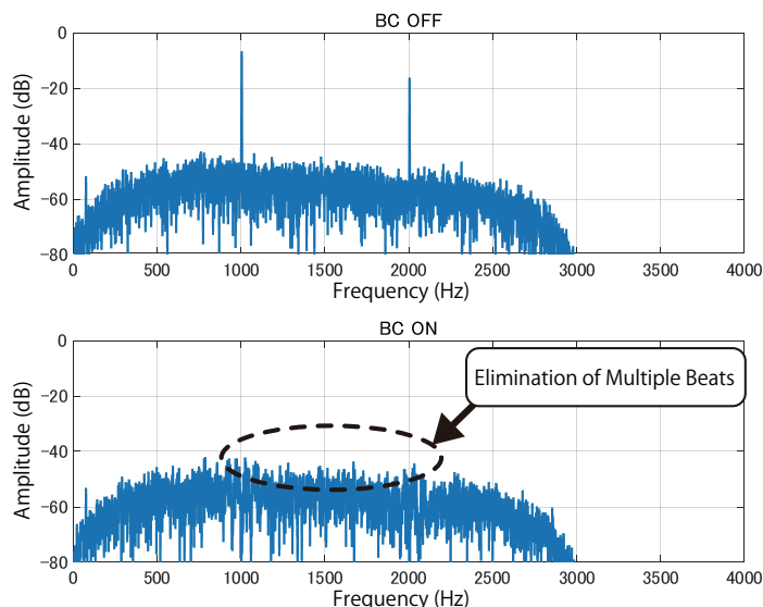
Fig. 50 Effect of Beat Canceled Elimination of Multiple Beats
