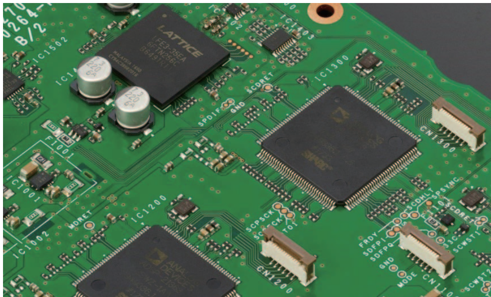
Fig. 30 Two SHARC Processors
