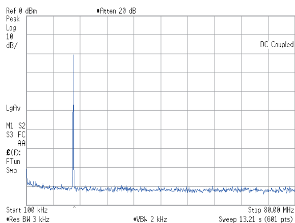
Fig. 24 DRV Output Characteristics 14.175 MHz -20 dBm
