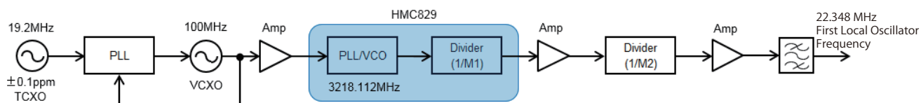
Fig. 25 Block Diagram of First Local Oscillator Signal (Reception of 14.1 MHz Signals)
