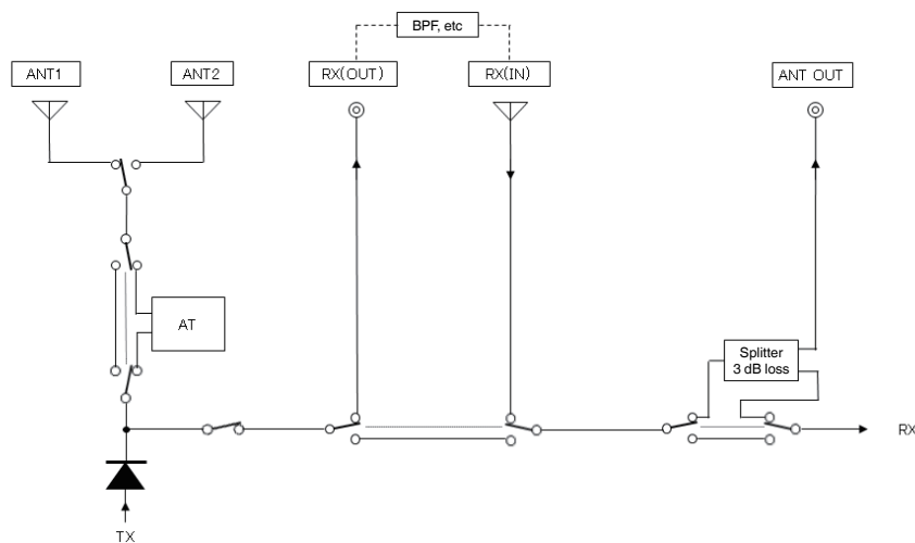
Fig. 29 Signaling Paths
