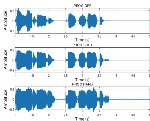
Fig. 58 IF Modulated Signal for Each IF Speech Processor Setting
